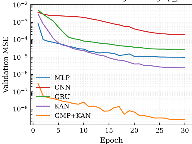
Validation MSE convergence — gmp_pa
