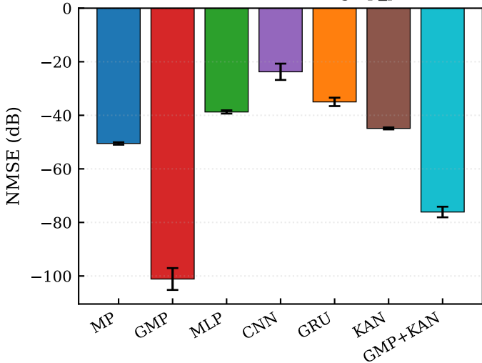
PA forward NMSE — gmp_pa
