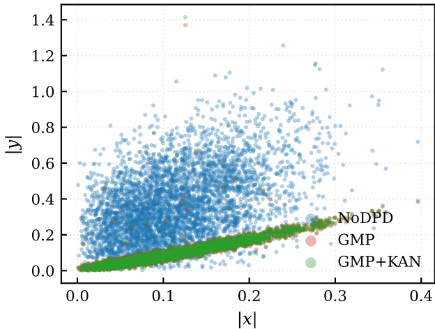
AM/AM after DPD — gmp_pa
