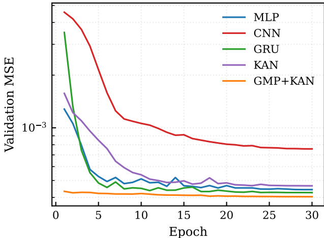
DPD training convergence — gmp_pa
