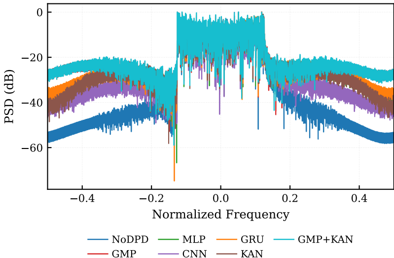
PSD after DPD — gmp_pa
