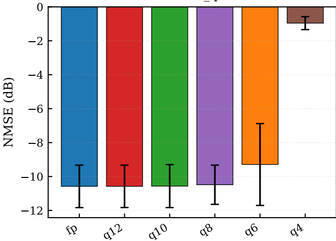
Ablation E_quant
