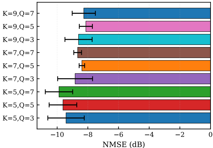
Ablation F_gmp_sweep
