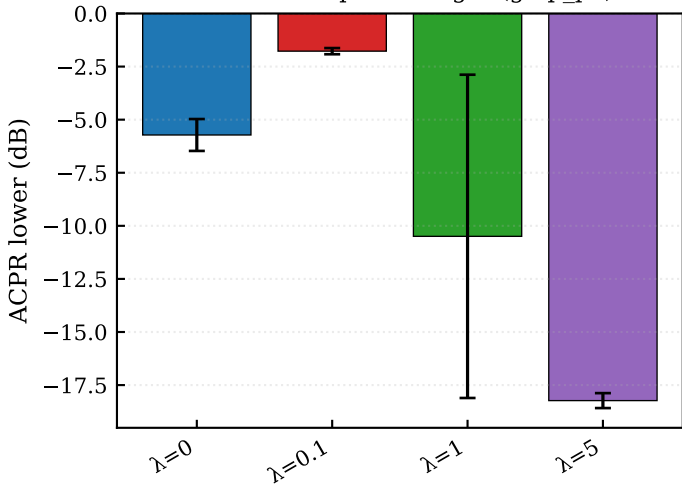
ACPR vs freq-loss weight (gmp_pa)
