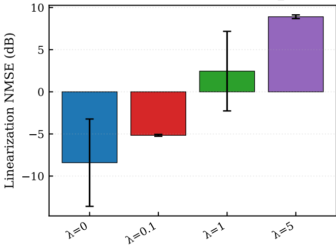
NMSE vs freq-loss weight (gmp_pa)
