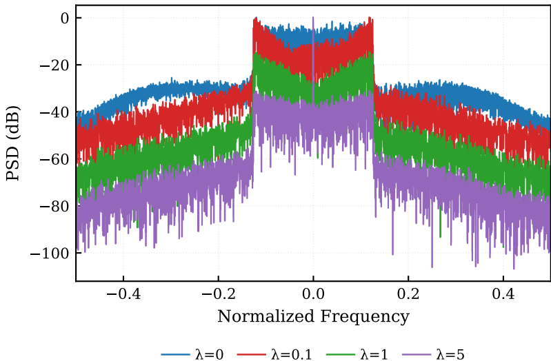
PSD: KAN-DPD vs frequency-loss weight \lambda (gmp_pa)
