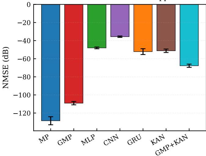
PA forward NMSE — rapp
