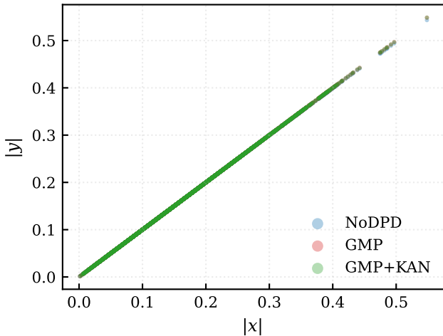
AM/AM after DPD — rapp
