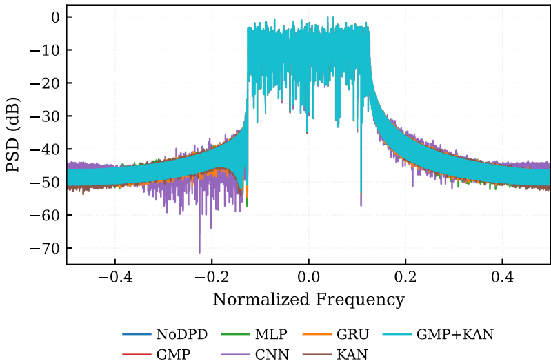
PSD after DPD — rapp
