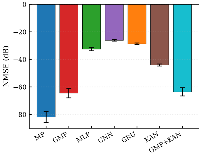
PA forward NMSE — saleh
