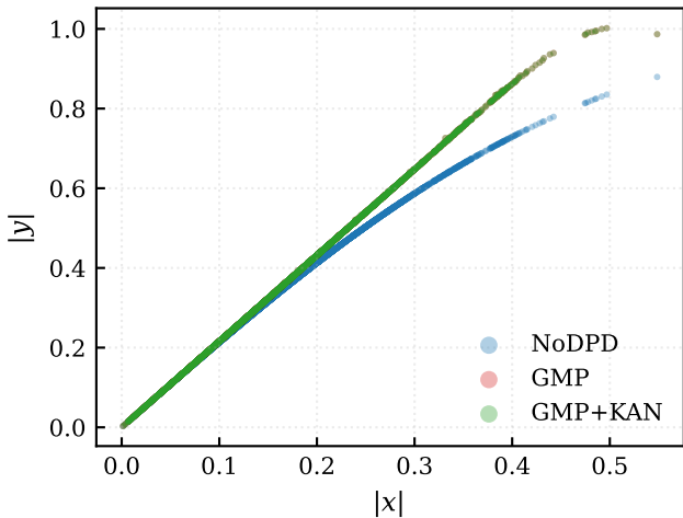
AM/AM after DPD — saleh
