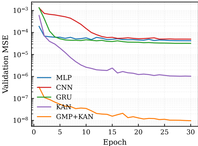
DPD training convergence — saleh
