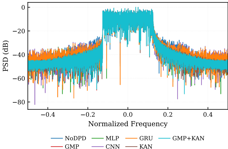
PSD after DPD — saleh
