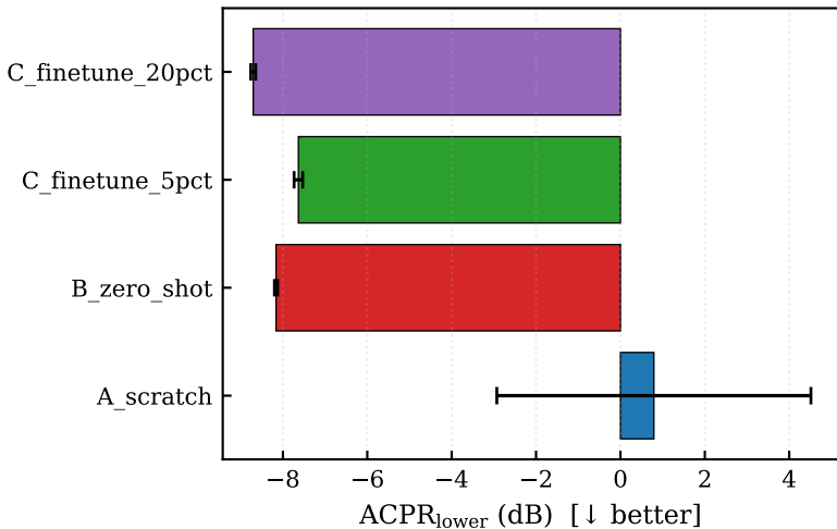
Sim \rightarrow Measured ACPR (DPA_160MHz.npz)
