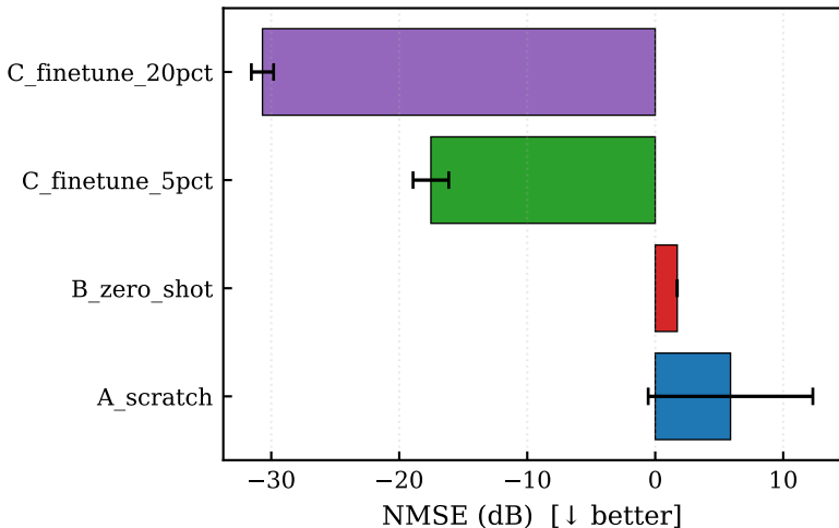
Sim \rightarrow Measured NMSE (DPA_160MHz.npz)
