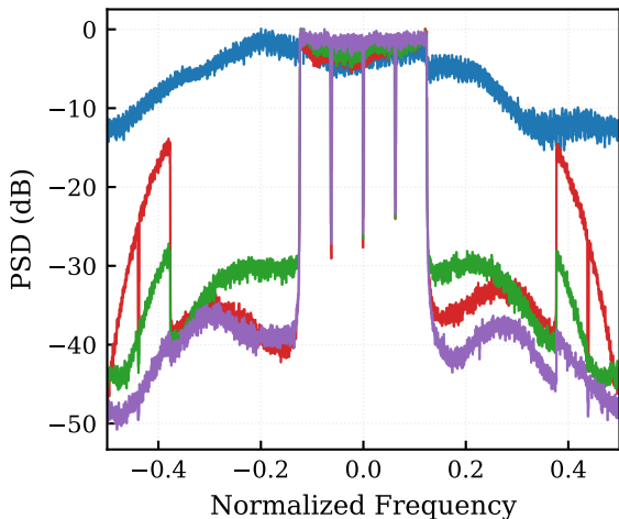
PSD by transfer strategy (DPA_160MHz.npz)
