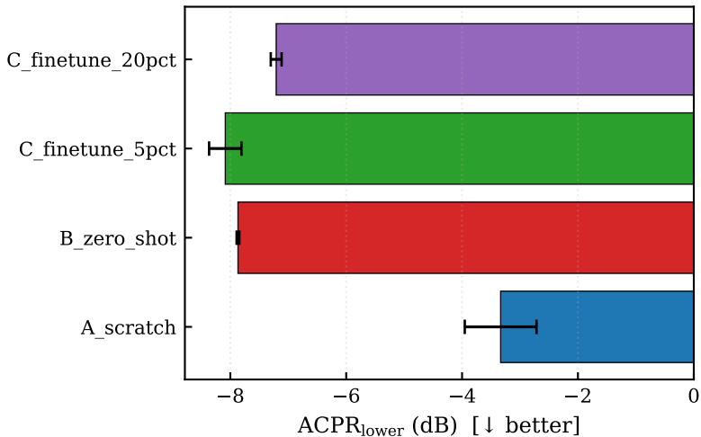
Sim \rightarrow Measured ACPR (DPA_200MHz.npz)
