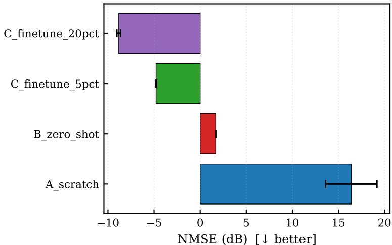
Sim \rightarrow Measured NMSE (DPA_200MHz.npz)
