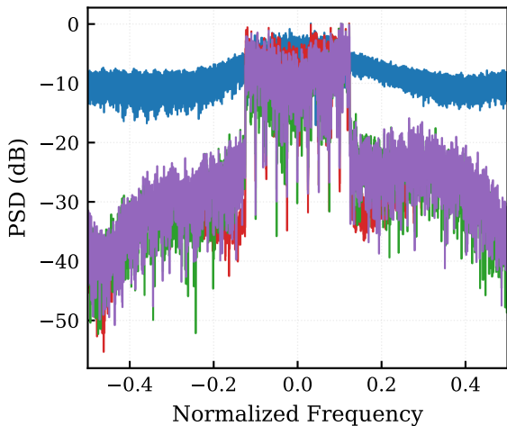
PSD by transfer strategy (DPA_200MHz.npz)
