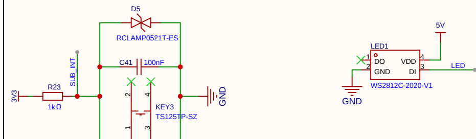
按键与LED
