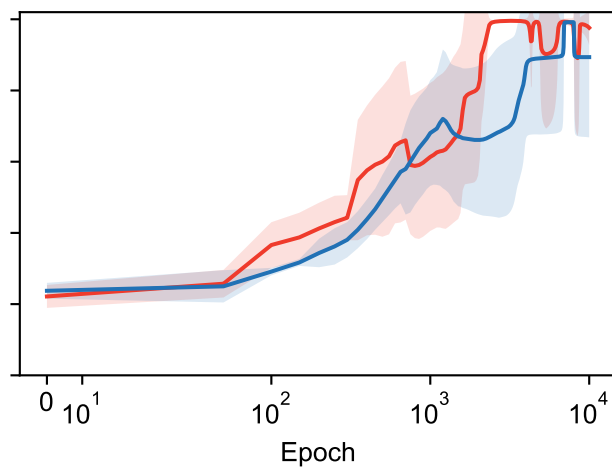
K = 97
