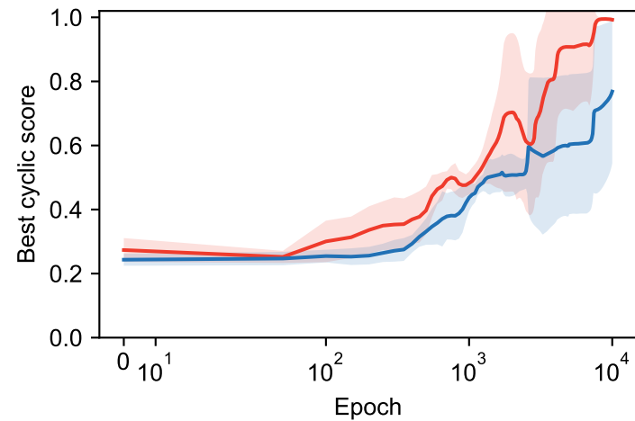
K = 79
