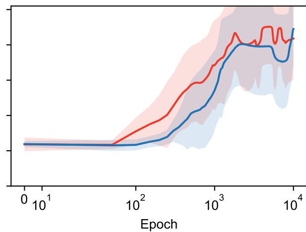
K = 113
