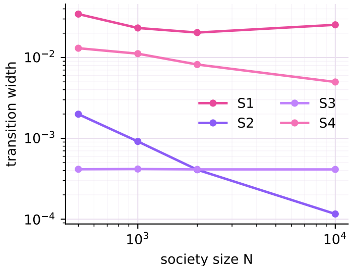
Transition width W(N)
