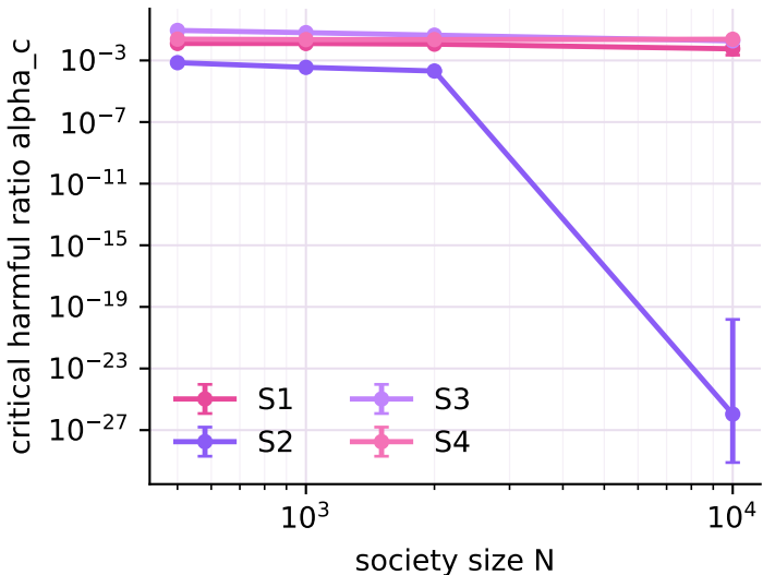
Critical ratio \alpha_c(N)
