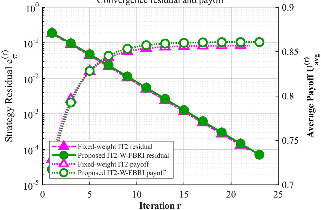
Convergence residual and payoff
