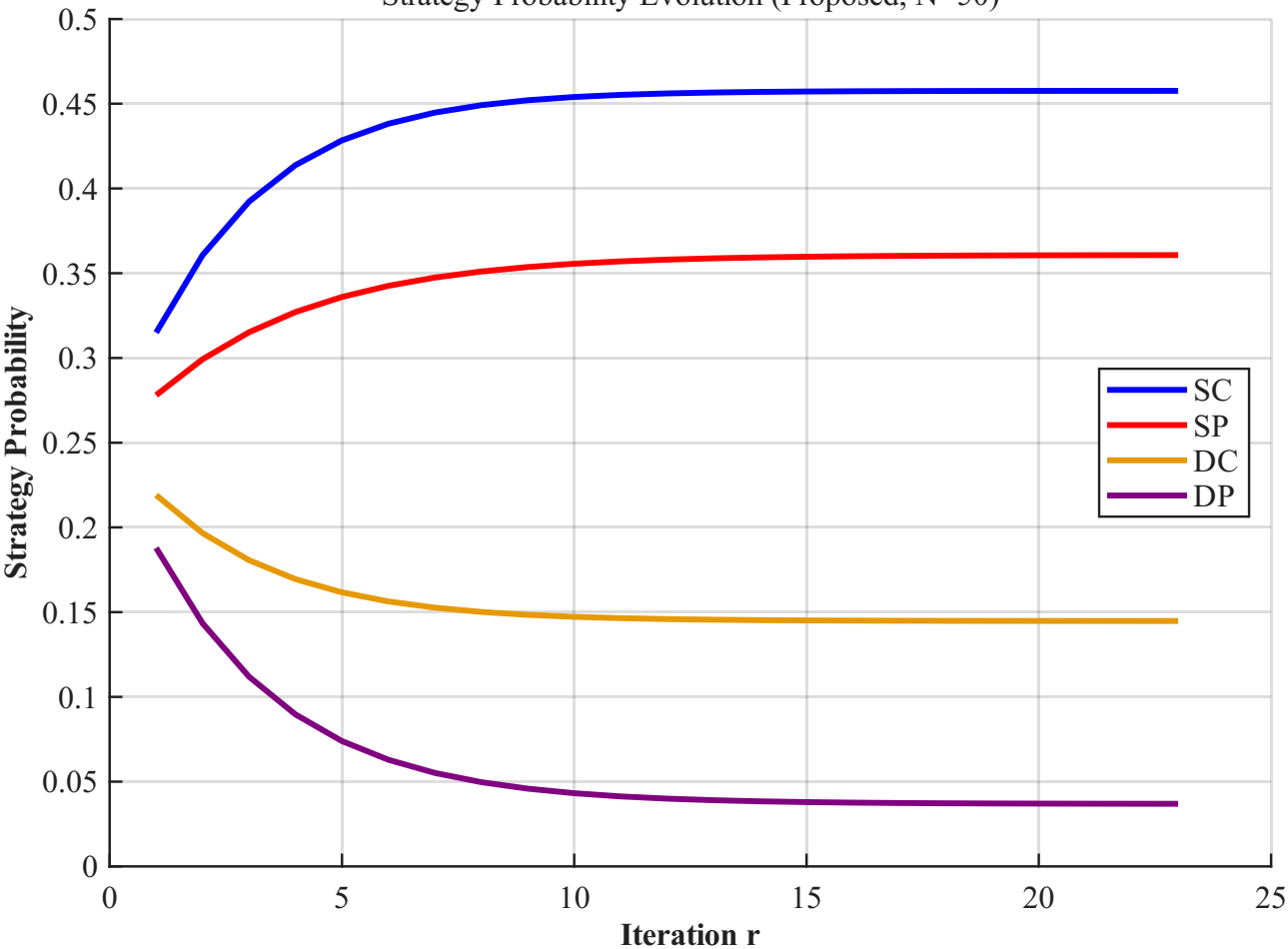
Strategy Probability Evolution (Proposed, N=50)
