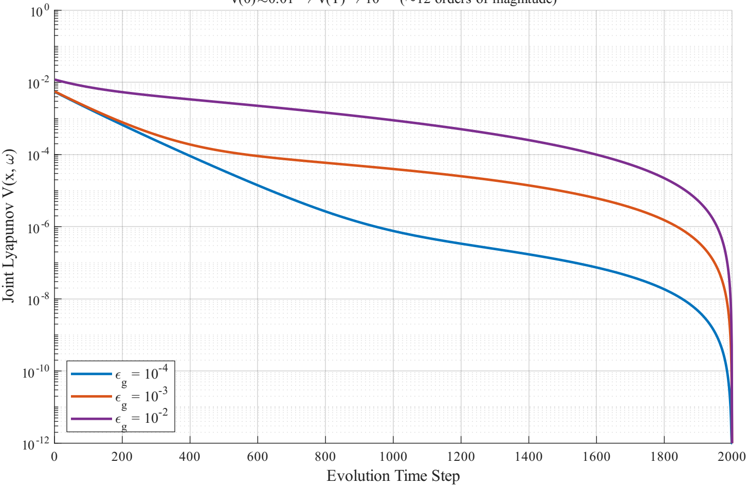
Joint Lyapunov Descent Along Coupled Trajectory (Eq. 4-42) V(0) \approx 0.01 \rightarrow V(T) \rightarrow 10^{-12} ( \sim 12 orders of magnitude)
