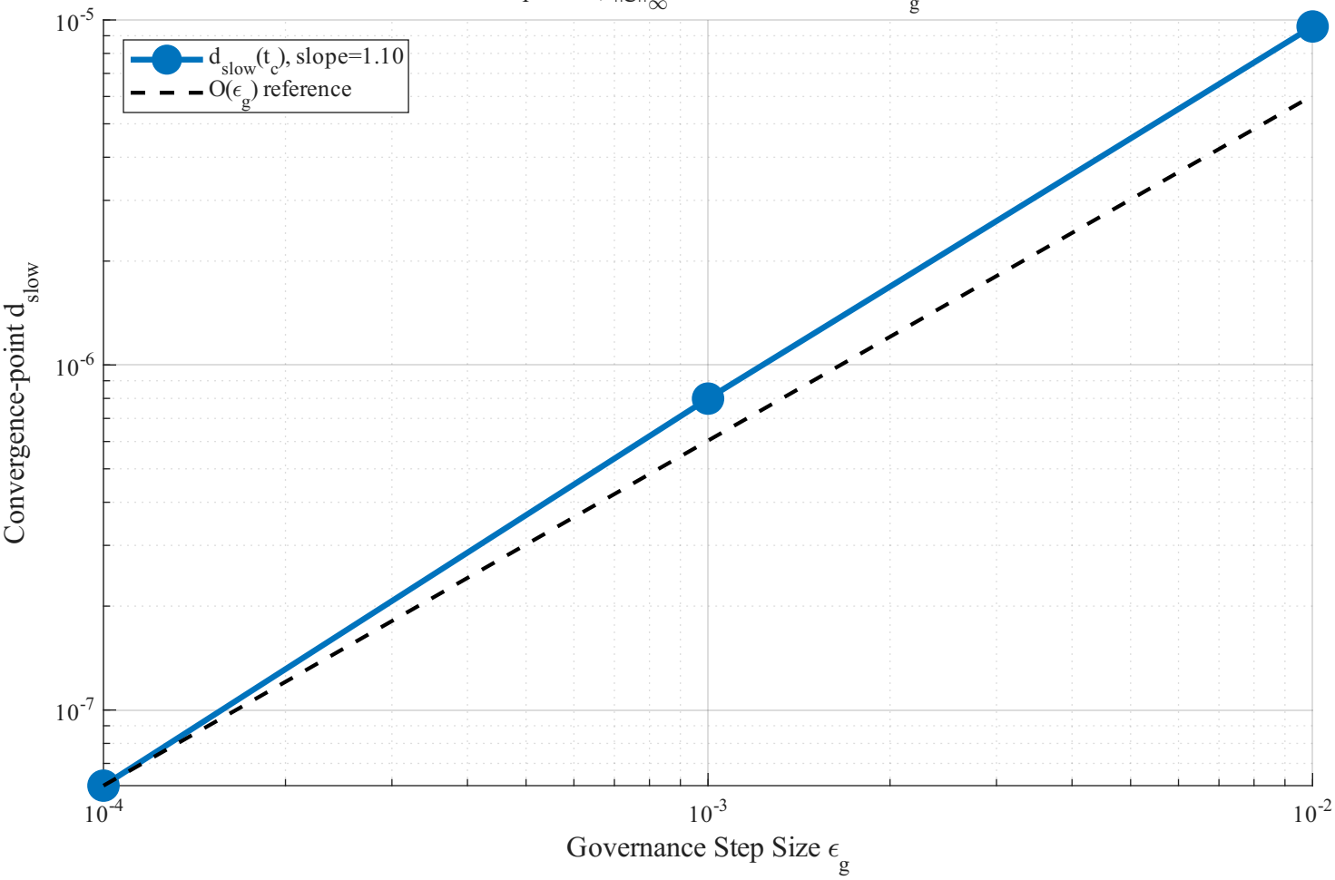
Matched Slow-Time Scaling After Governance Convergence slope 1.10, \|g\|_\infty < 1e-03 for all tested \epsilon_g
