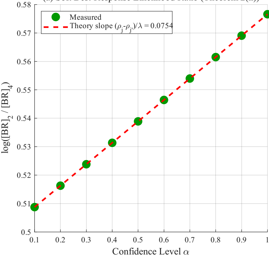
(a) Soft Best-Response Likelihood Ratio (Theorem 2(ii))
