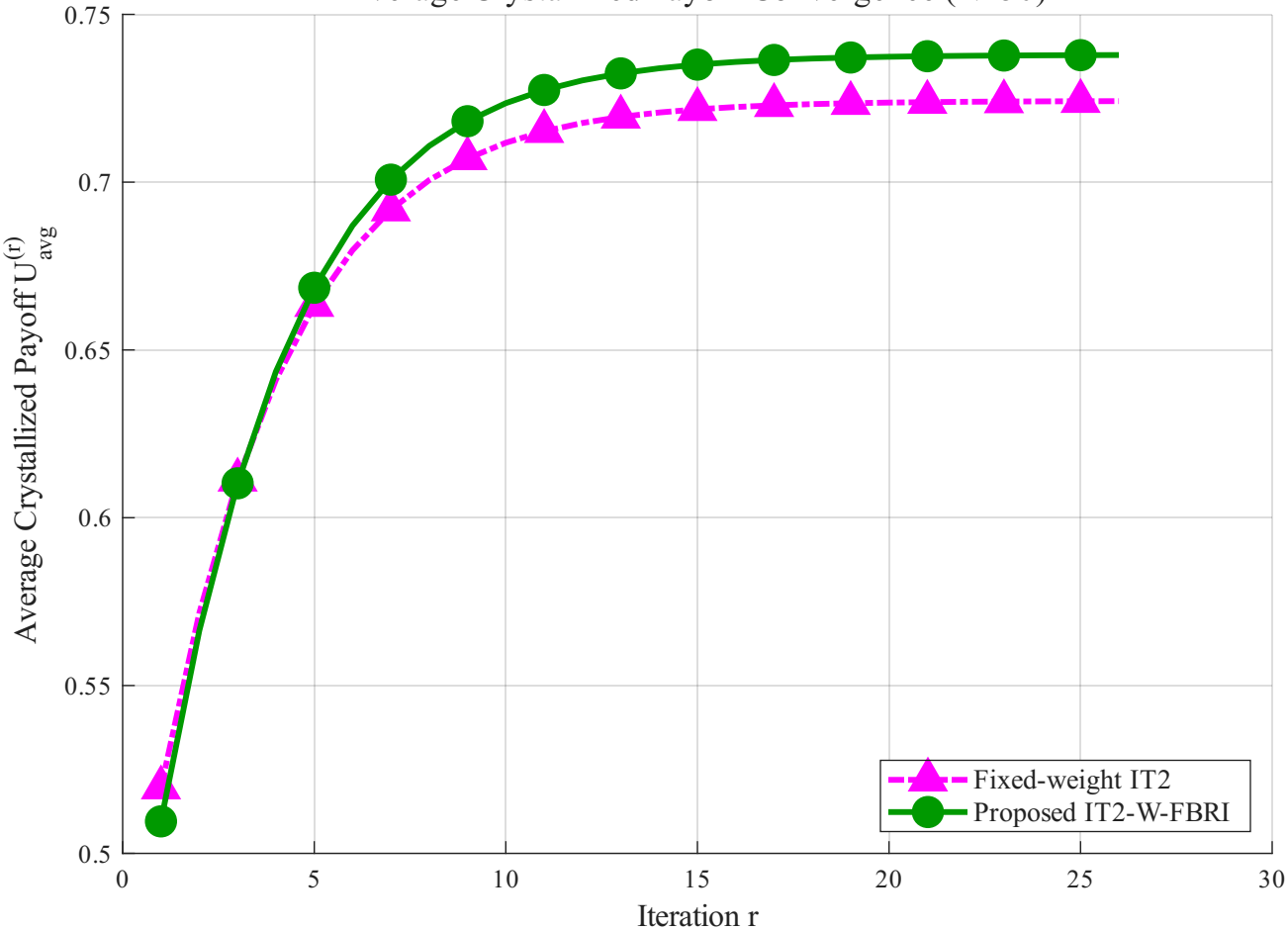
Average Crystallized Payoff Convergence (N=50)
