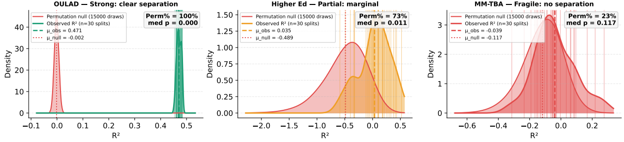
Figure 4. Empirical permutation null vs. observed linear R^2 for three representative datasets. The red density is the pooled empirical null distribution from 500 permutation draws on each of 30 random 80/20 splits (15,000 values total per dataset); the coloured density is the observed-label R^2 across the same 30 splits, with vertical ticks marking individual splits and dashed/dotted lines showing the means. OULAD shows clean separation (Perm% = 100%), Higher Ed is borderline but below the pass threshold (Perm% = 73%), and MM-TBA shows substantial overlap (Perm% = 23%, median p = 0.117).
