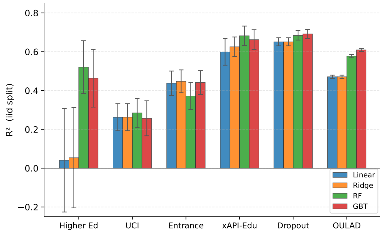
(a) iid Performance
