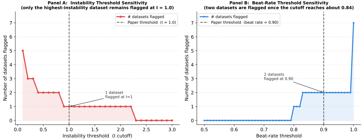
Fig S3: Threshold-sensitivity sweeps for the two operational cutoffs used in the audit. Panel (a) varies the instability cutoff over I \in [0.1, 3.0] and reports the number of datasets that would be flagged as failing split instability; the paper's choice of I = 1.0 flags one dataset (MM-TBA, with linear I = 2.21 ), while more lenient cutoffs below about 0.9 additionally flag Higher Ed. Panel (b) varies the beat-rate cutoff over [0.5, 1.0] ; the paper's choice of 0.90 flags two datasets, whereas more lenient cutoffs below about 0.84 reduce the flagged count. The main qualitative pattern remains unchanged: MM-TBA is always the weakest case, and Higher Ed is the only borderline dataset near the operational thresholds.
