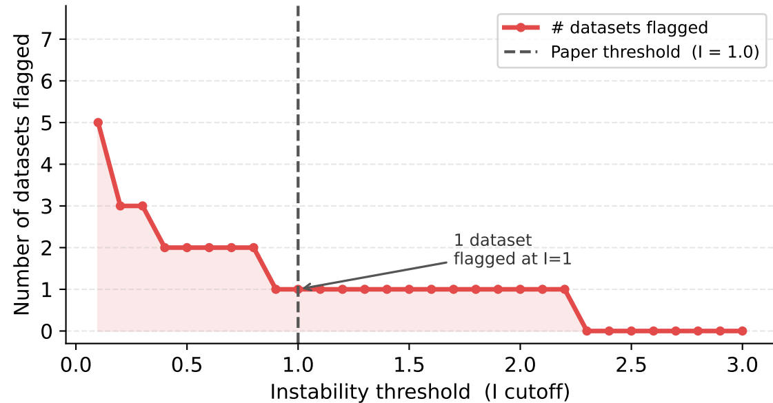
(a) Instability Threshold Sensitivity (only the highest-instability dataset remains flagged at I = 1.0 )
