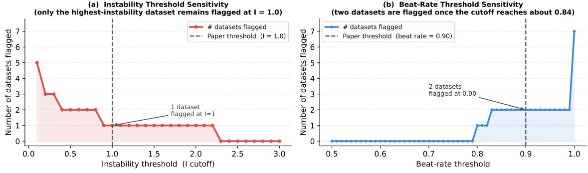
Fig S3: Threshold-sensitivity sweeps for the two operational cutoffs used in the audit. Panel (a) varies the instability cutoff over I \in [0.1, 3.0] and reports the number of datasets that would be flagged as failing split instability; the paper's choice of I = 1.0 flags one dataset (MM-TBA, with linear I = 2.21 ), while more stringent cutoffs below about 0.9 additionally flag Higher Ed. Panel (b) varies the beat-rate cutoff over [0.5, 1.0] ; the paper's choice of 0.90 flags two datasets, whereas more lenient cutoffs below about 0.84 reduce the flagged count. The main qualitative pattern remains unchanged: MM-TBA is always the weakest case, and Higher Ed is the only borderline dataset near the operational thresholds.
