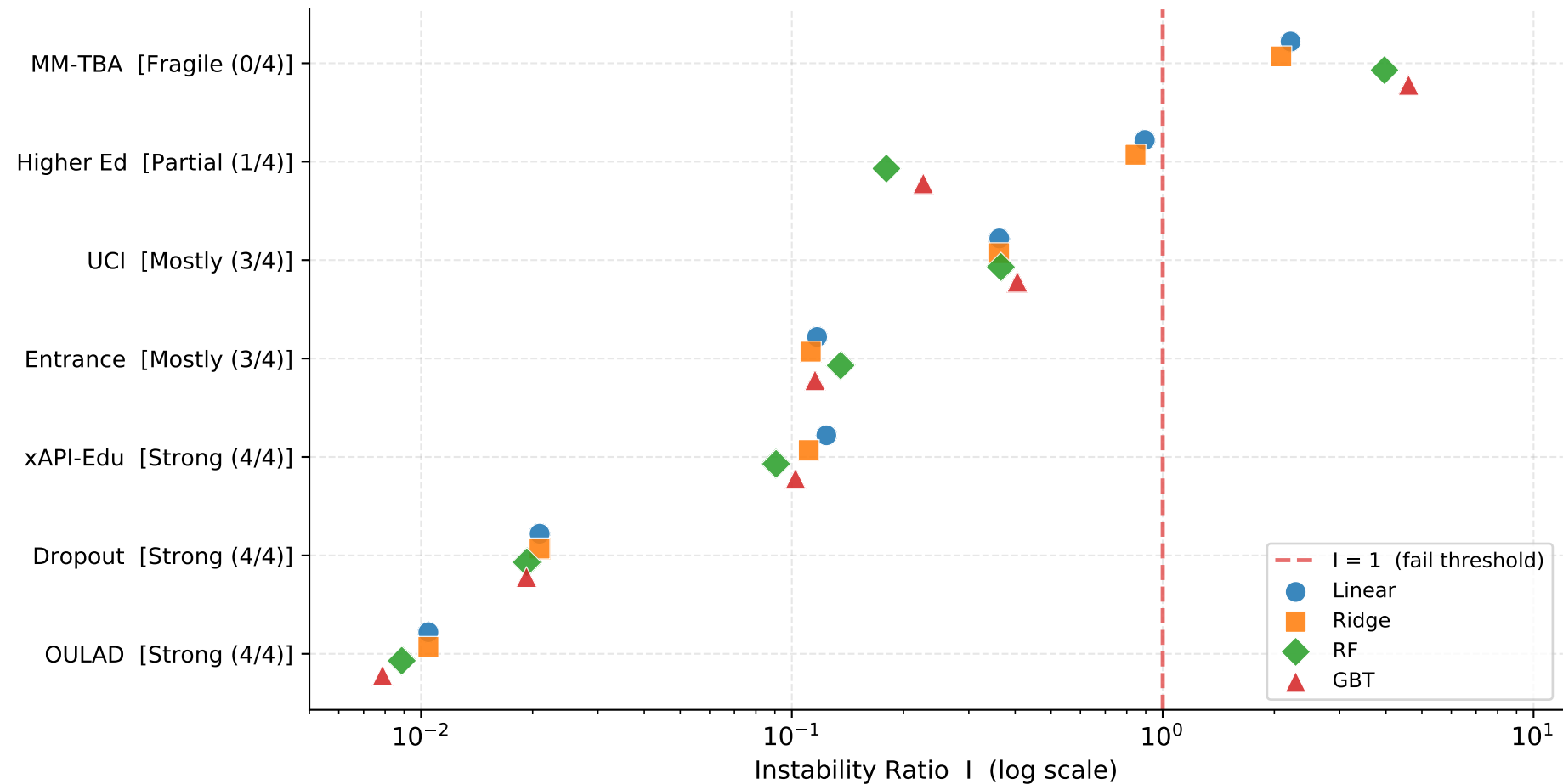
Split Instability Across Seven Datasets and Four Models MM-TBA Ensemble Models Are Extreme Outliers; Strong Datasets Cluster near I = 0.01
