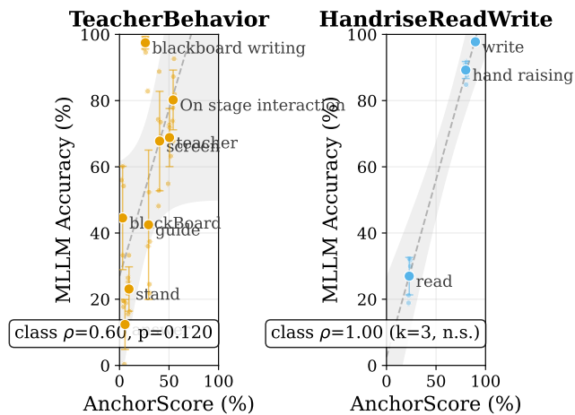
FIGURE A1. Per-dataset correlation between AnchorScore and MLLM accuracy for TeacherBehavior ( k = 8 , left) and HandriseReadWrite ( k = 3 , right). Class means (large markers) are shown with \pm 1 SD error bars across the six MLLMs; the dashed OLS line, its 95% confidence band, and the reported \rho are all computed on class means ( n = k per dataset). Individual MLLM points are jittered horizontally ( \pm 1.5\% ) for visibility. BowTurnHead ( k = 2 ) is omitted as Spearman on two points is uninformative; for k < 5 the p -value is suppressed.
