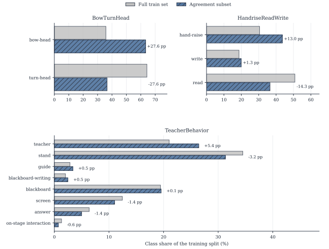
FIGURE 5. Class-composition shift between the full training split and the agreement subset for each dataset. Labels on the agreement bars report percentage-point change relative to the full training distribution, making the direction and magnitude of selection bias explicit.
