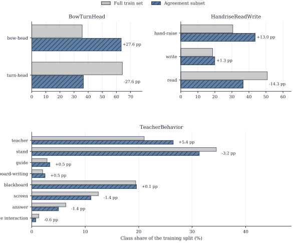
FIGURE 5. Class-composition shift between the full training split and the agreement subset for each dataset. Labels on the agreement bars report percentage-point change relative to the full training distribution, making the direction and magnitude of selection bias explicit.
