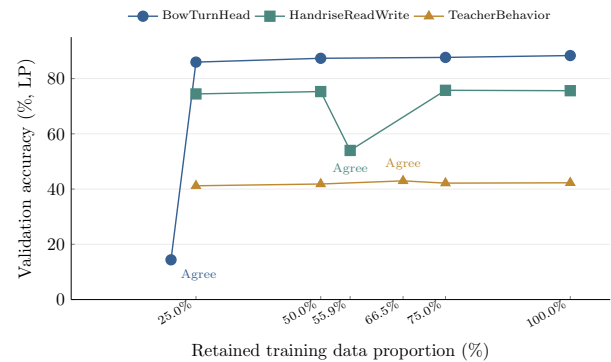
FIGURE 6. Retention-ratio curves for BowTurnHead, HandriseReadWrite, and TeacherBehavior under linear probing with unfiltered pseudo-labels (None strategy), augmented with the agreement-filtered endpoint (labelled “Agree”). All plotted points are fixed-seed diagnostic runs (seed 42), whereas Table 8 reports repeated-seed LP means for the main downstream comparison. The x-axis reports training-set retention rates, whereas Table 5 reports validation-set retention rates for annotation quality. Random subsampling remains stable above the critical retention threshold for all three datasets. The agreement-selected endpoint falls far below the random-retention trend for BowTurnHead and HandriseReadWrite, whereas TeacherBehavior shows only a small positive deviation.
