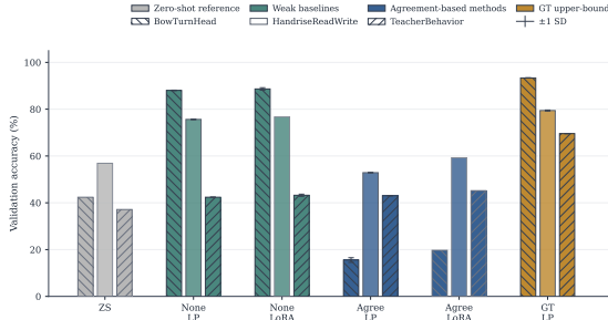
FIGURE 4. Overview of the full evaluation matrix. The plot includes the three zero-shot baselines and all 18 CLIP fine-tuning conditions formed by three datasets, three label sources, and two fine-tuning methods. Solid bars denote repeated or replicated conditions; hatched bars denote single-run references; error bars show \pm 1 SD when available. ZS = zero-shot CLIP; LP = linear probing; LoRA = low-rank adaptation; Agree = agreement-filtered pseudo-labels. Here, ZS bars follow the baseline zero-shot setting used in Table 7 under the same bbox-crop validation protocol; LP bars use repeated-seed means, whereas LoRA bars combine the targeted five-seed replication values for BowTurnHead and TeacherBehavior under None and GT with protocol-matched seed-42 references elsewhere. Prompt-ensemble zero-shot values are reported separately in the selective-analysis section.
