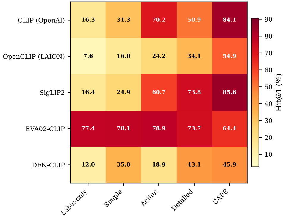
TeacherBehavior (8 classes)
