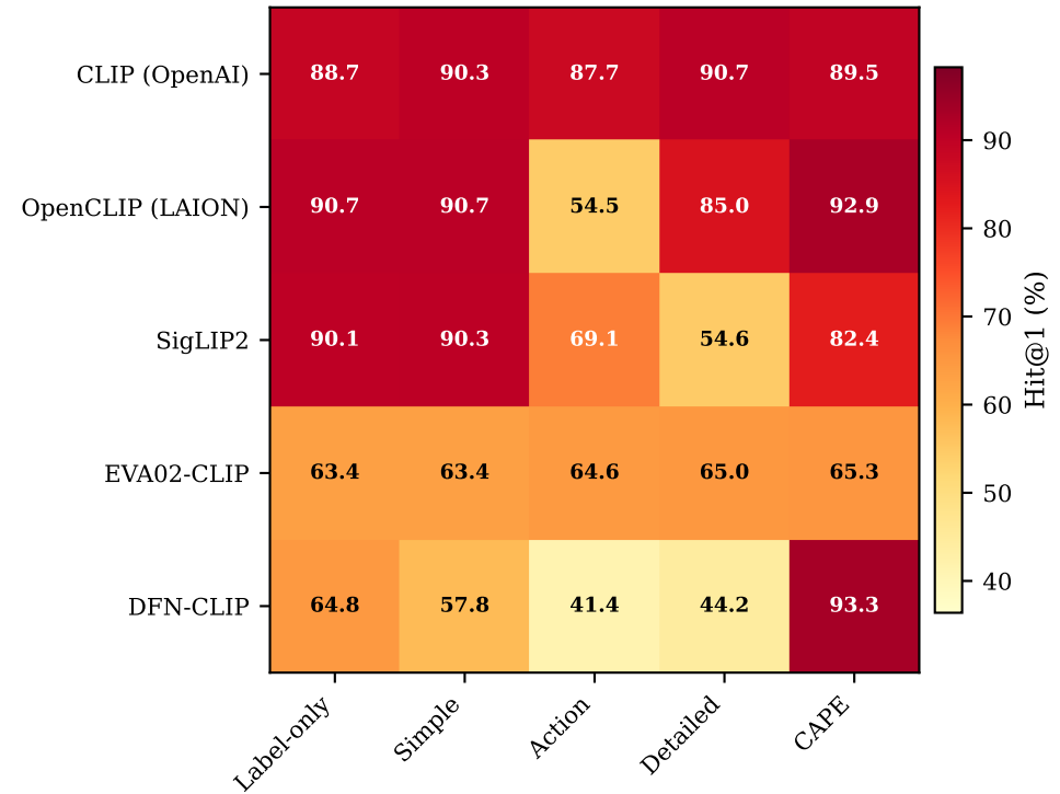
BowTurnHead (2 classes)
