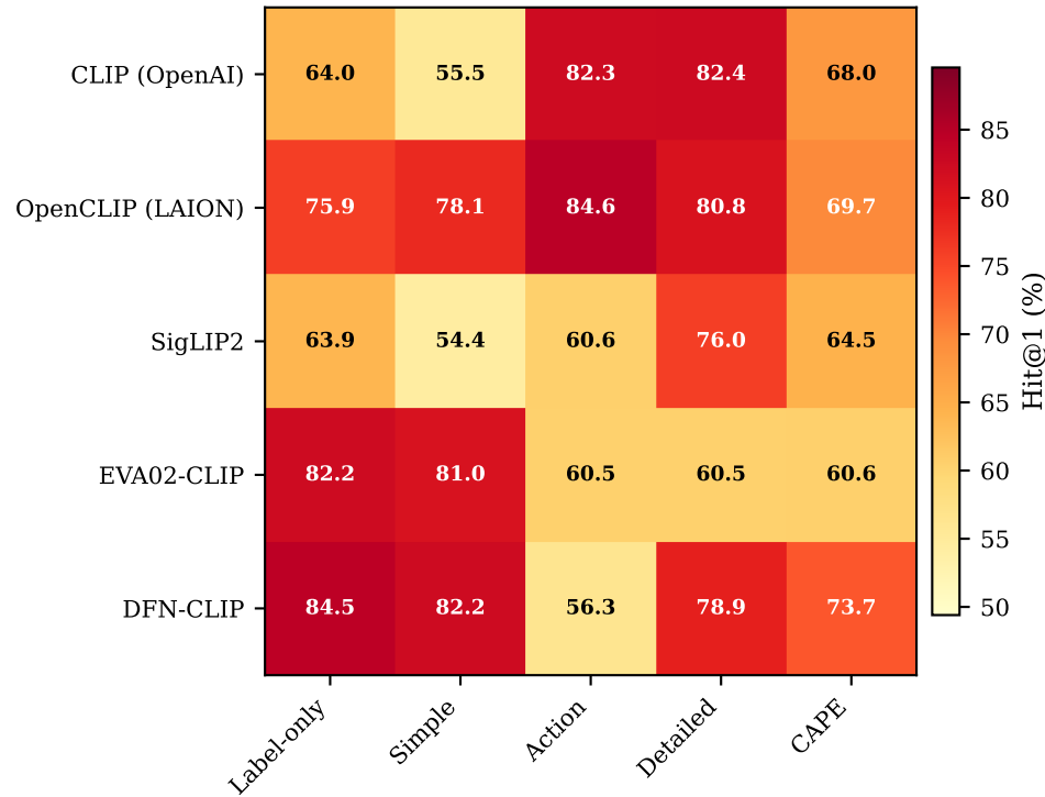
HandriseReadWrite (3 classes)
