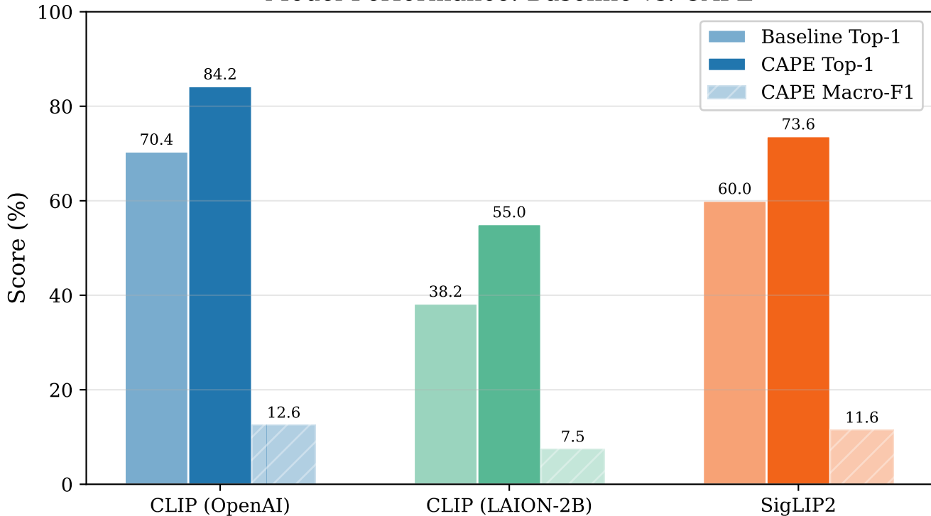
Model Performance: Baseline vs. CAPE
