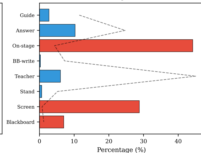
DFN-CLIP (cape)
