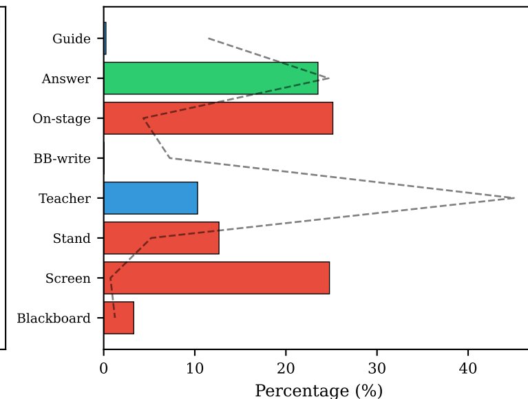
DFN-CLIP (cape)
