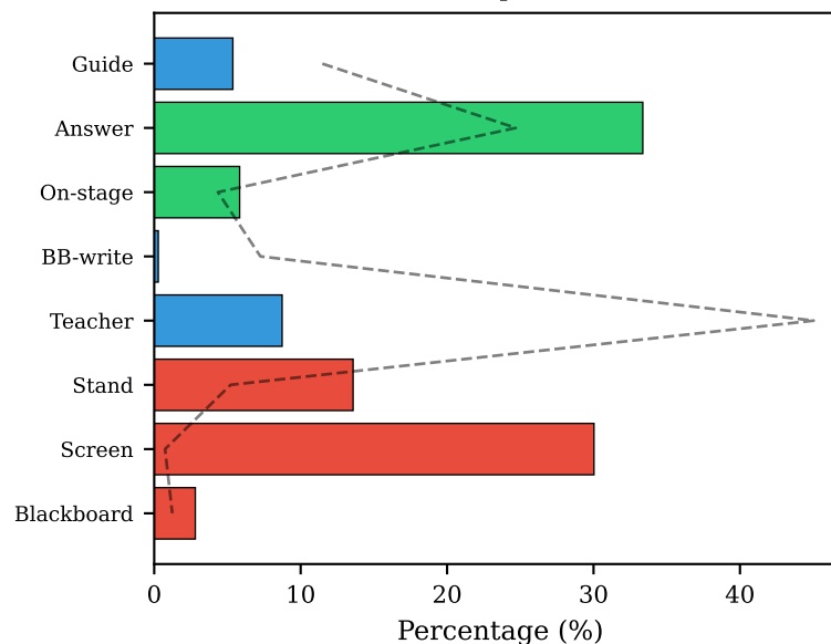
EVA02-CLIP (cape)
