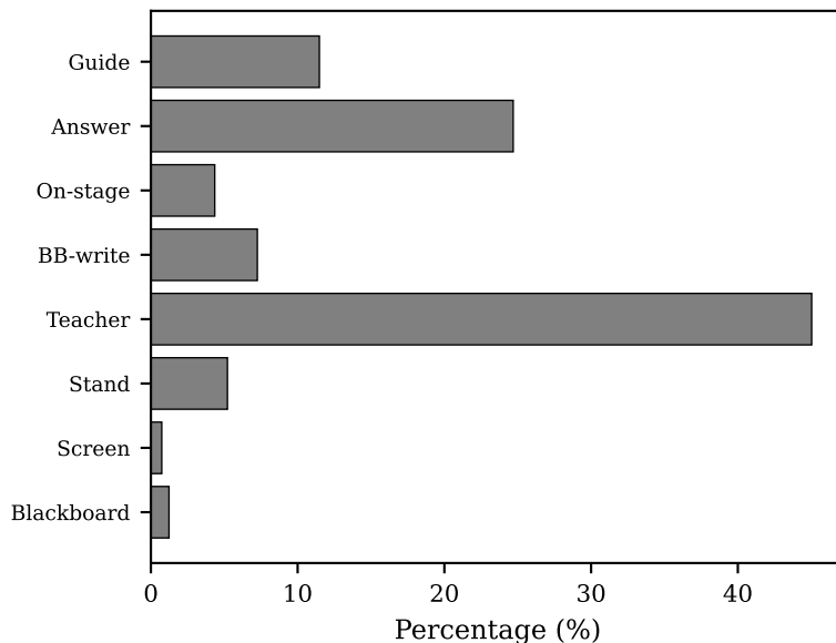
SigLIP2 (cape)
