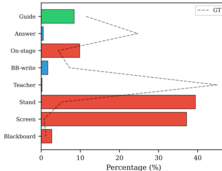
EVA02-CLIP (cape)
