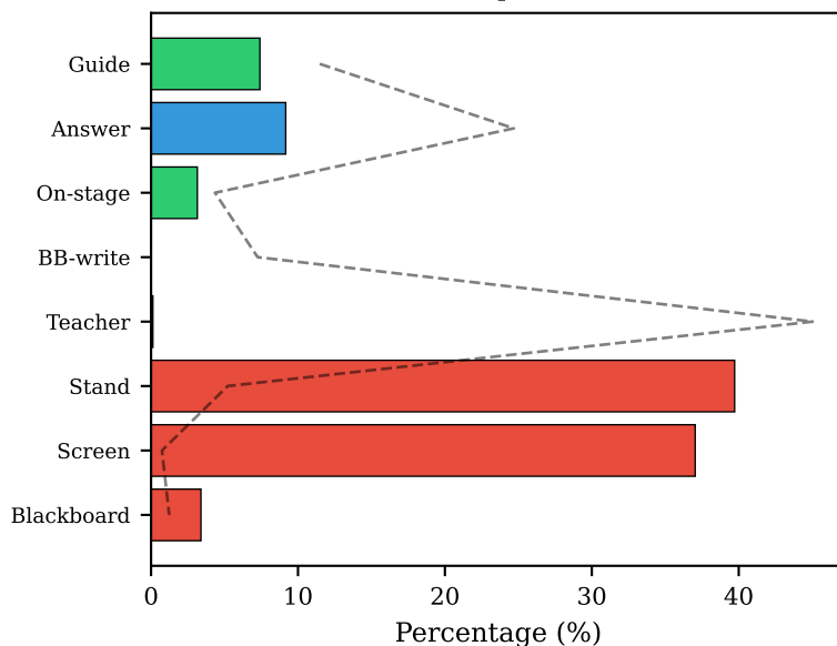
SigLIP2 (cape)
