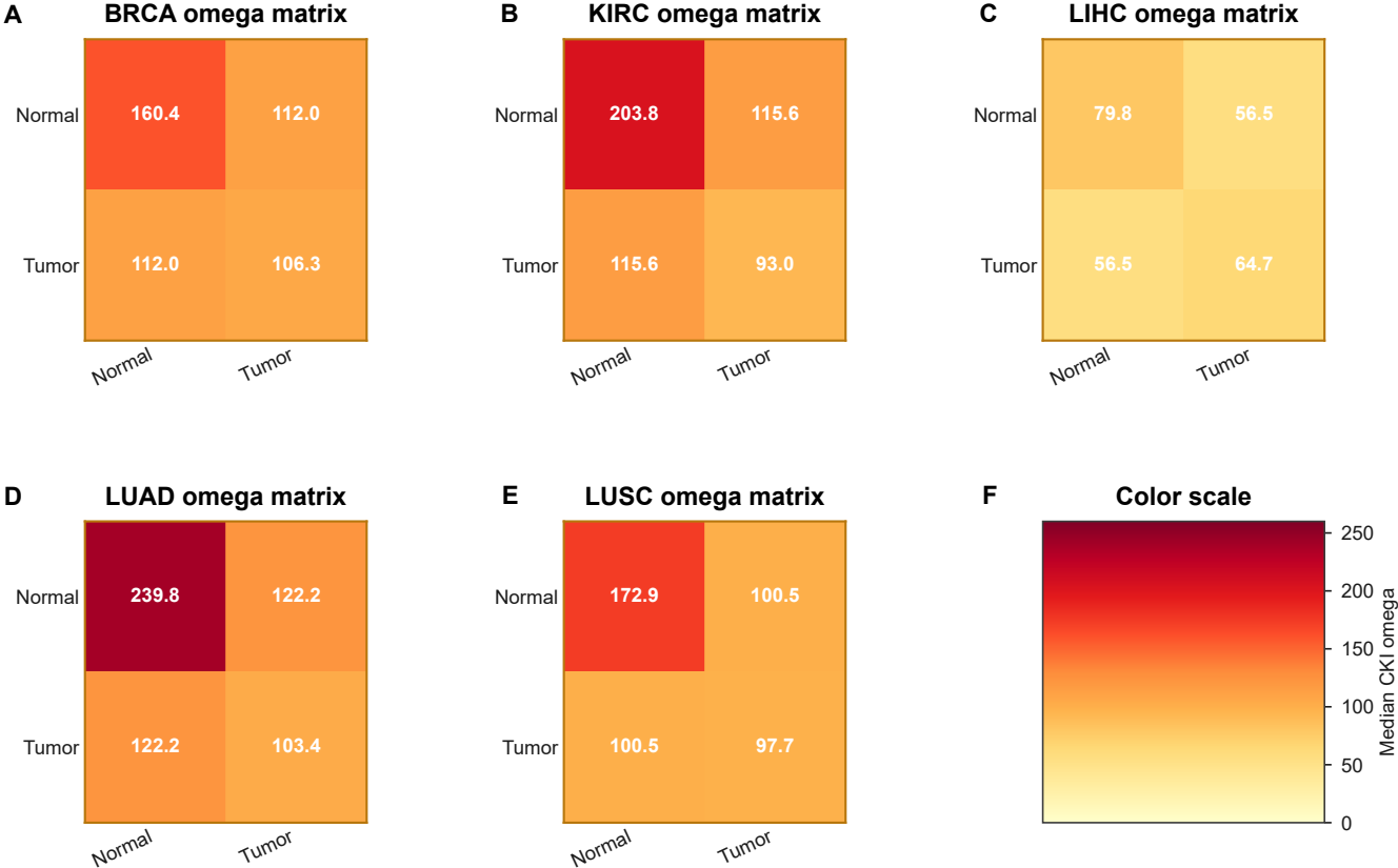
Supplementary Figure S4. TCGA per-cancer CKI omega matrices (Normal vs Tumor; median \omega shown).
