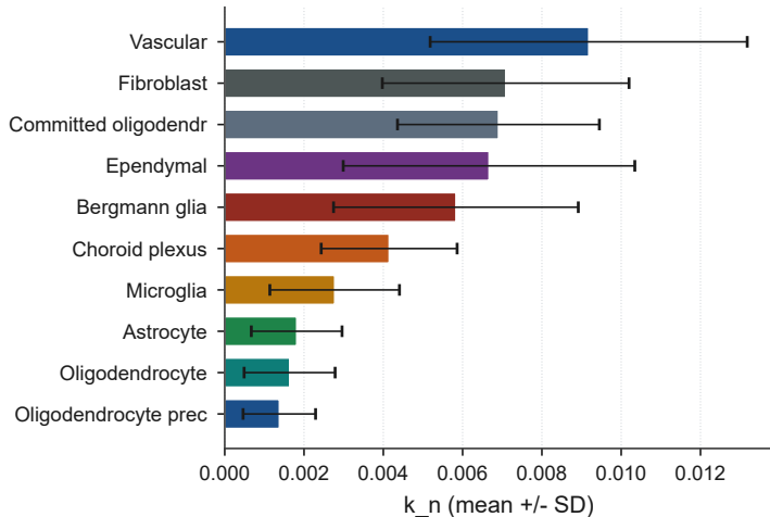
A. Per-pair k_n by cell type (brain)
