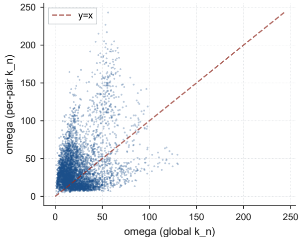
B. Per-pair vs global k_n omega ( \rho=0.142 )
