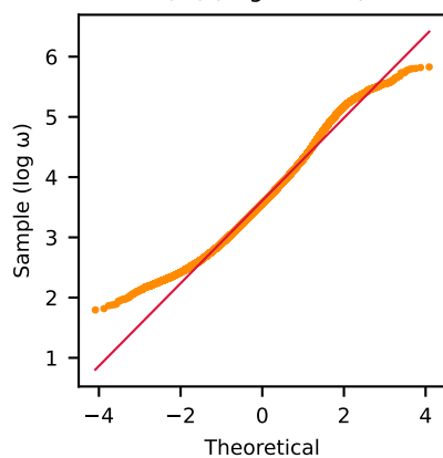
Q-Q (Log-Normal)
