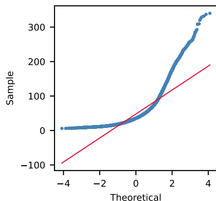
Q-Q (Log-Normal)
