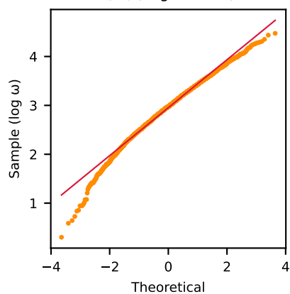
Q-Q (Log-Normal)
