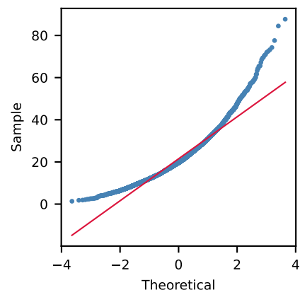
Q-Q (Log-Normal)
