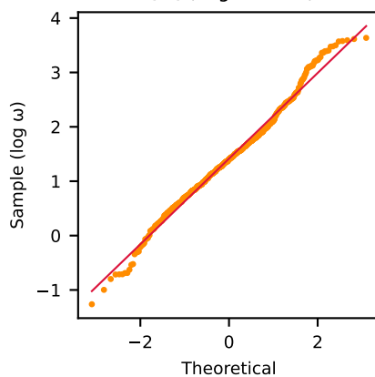
Q-Q (Log-Normal)
