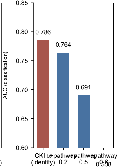
(C) k_f component weight sweep
