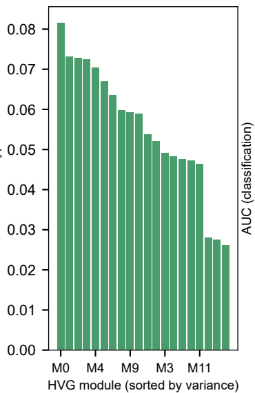
(B) Prevalence distributed across HVG modules
