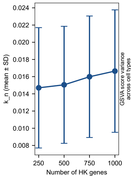
(A) k_n stability vs. HK gene set size
