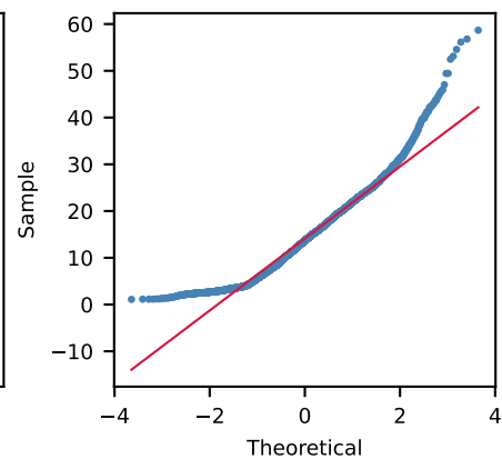
Q-Q (Log-Normal)
