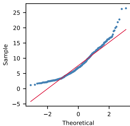
Q-Q (Log-Normal)
